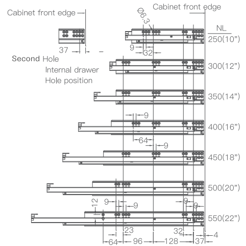
Hole position
