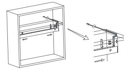
side install
